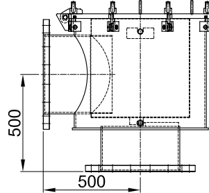
DN 500
