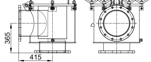
DN 300
