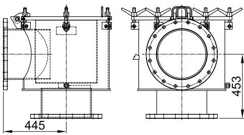
DN 350
