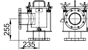
DN 125
