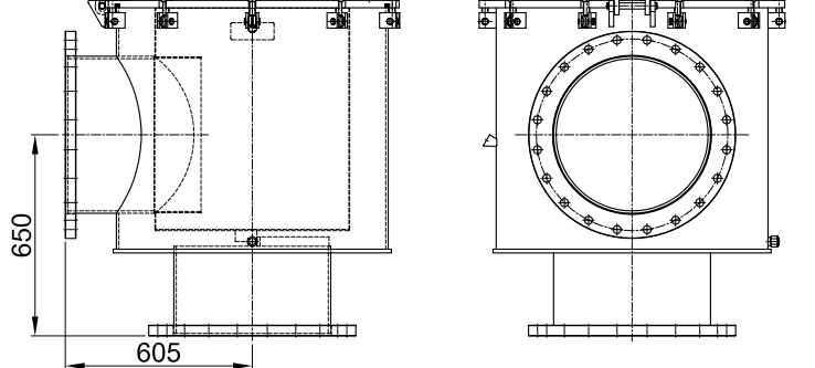
DN 500
